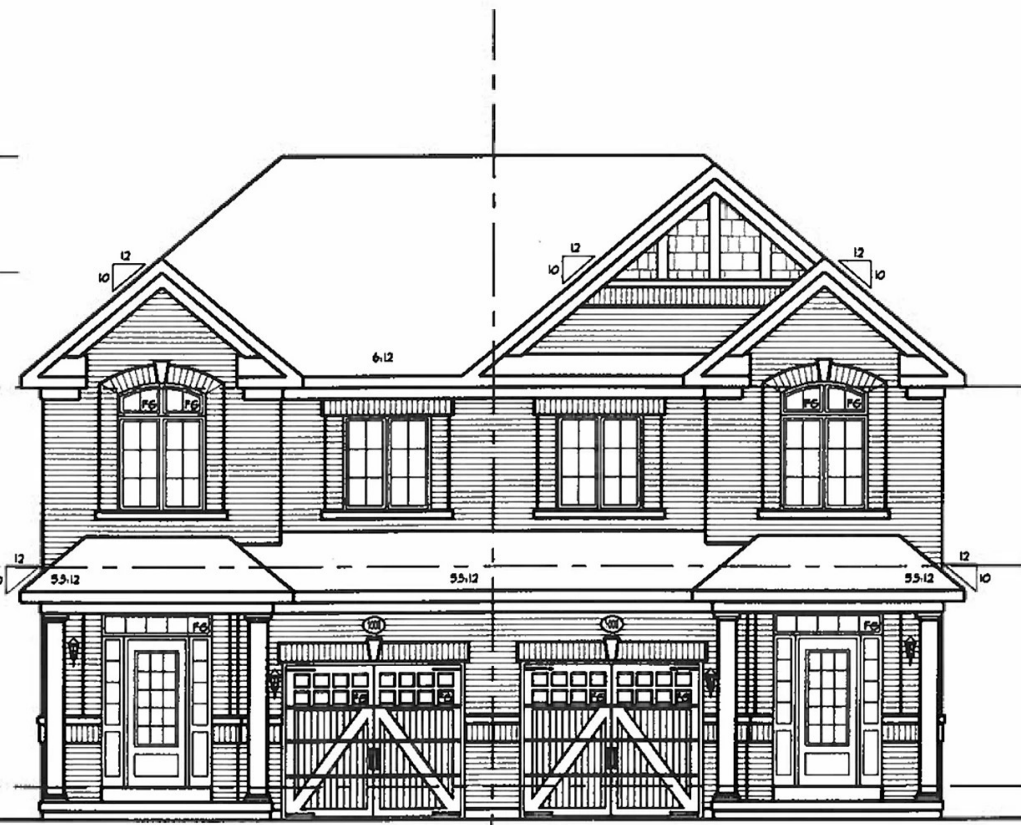
FRONT ELEVATION 'A-1'
