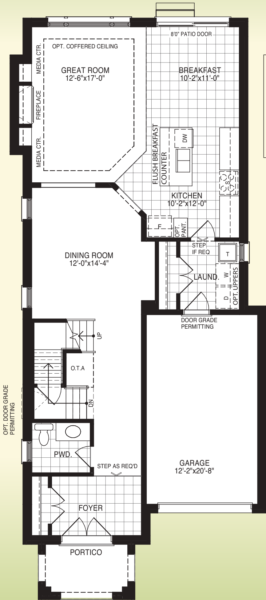
Ground Floor Plan Elev. A
