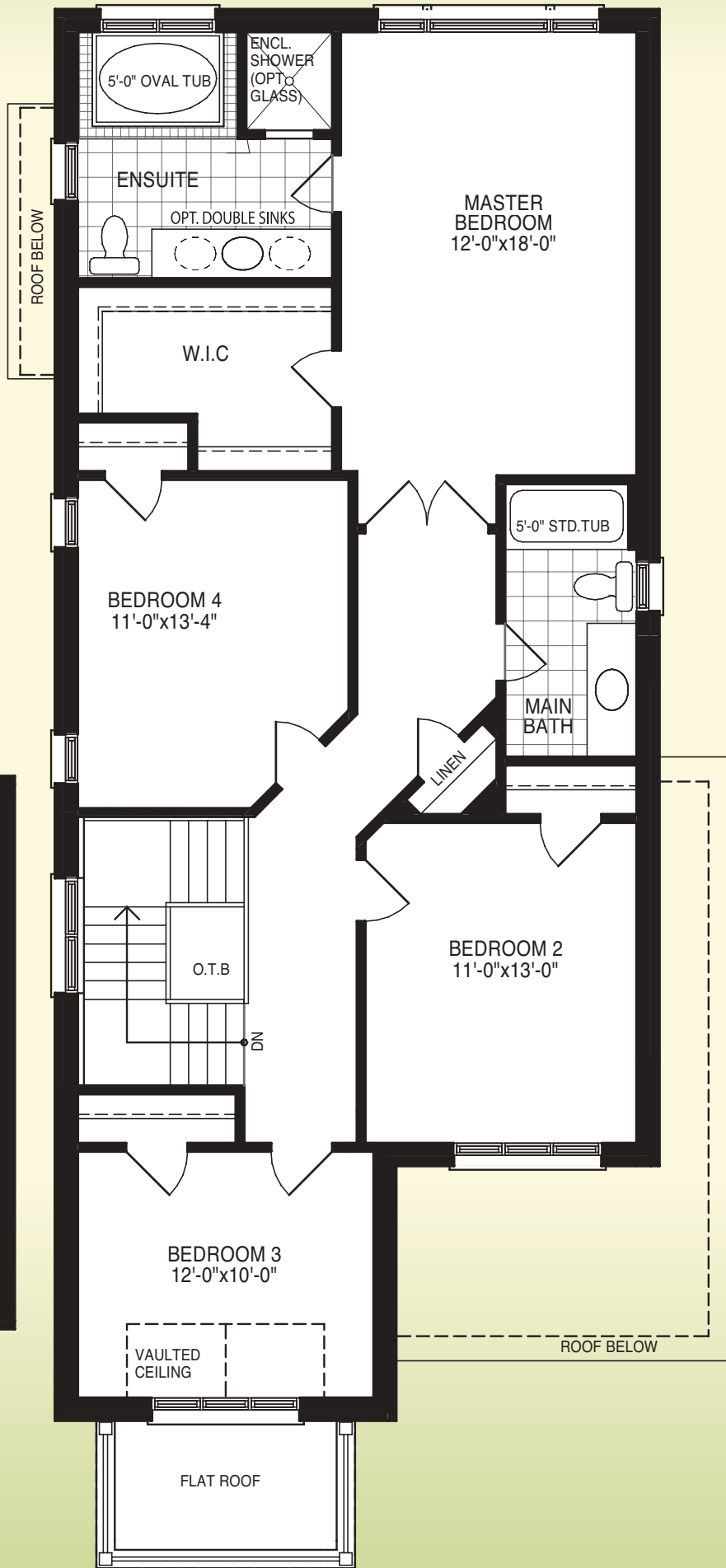
Second Floor Plan Elev. A
