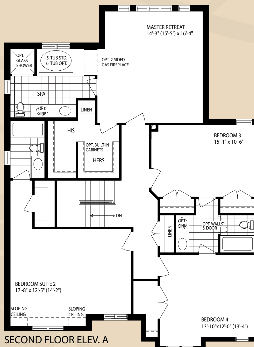
SECOND FLOOR ELEV. A 5 BEDROOM PLAN
