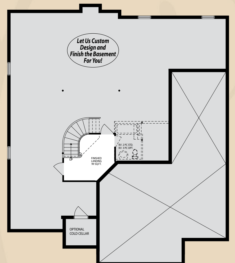
BASEMENT ELEV. A (4 CAR GARAGE) (SHADED AREA IS UNFINISHED SPACE)
