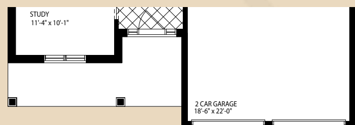
MAIN FLOOR ELEV. B FOR 50' LOTS (2 CAR GARAGE)
