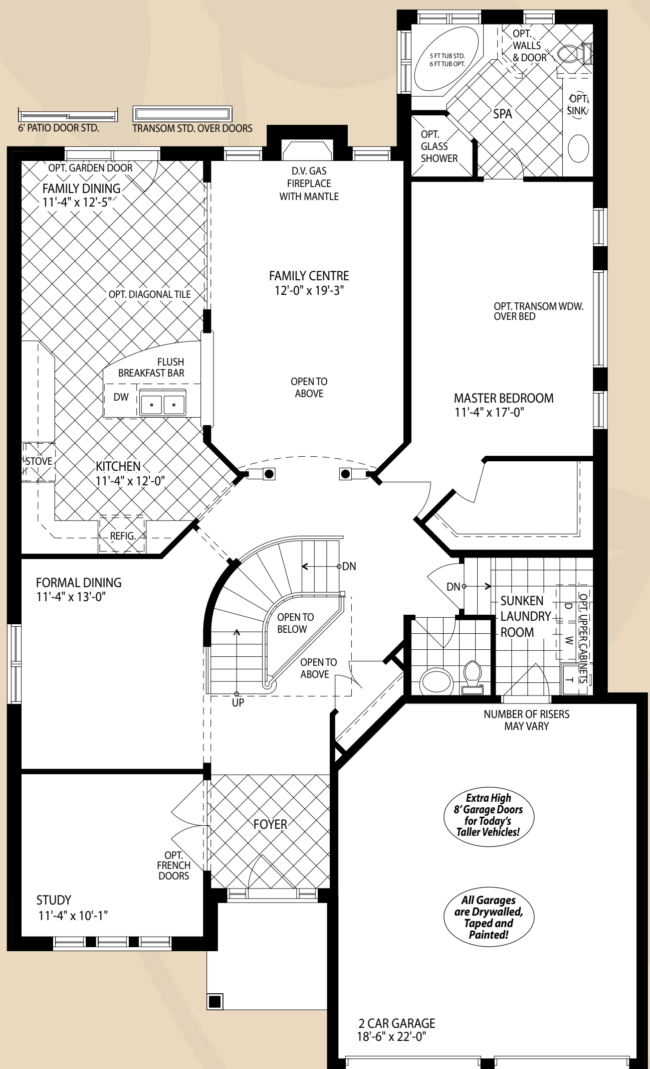
MAIN FLOOR ELEV. A FOR 50' LOTS (2 CAR GARAGE)
