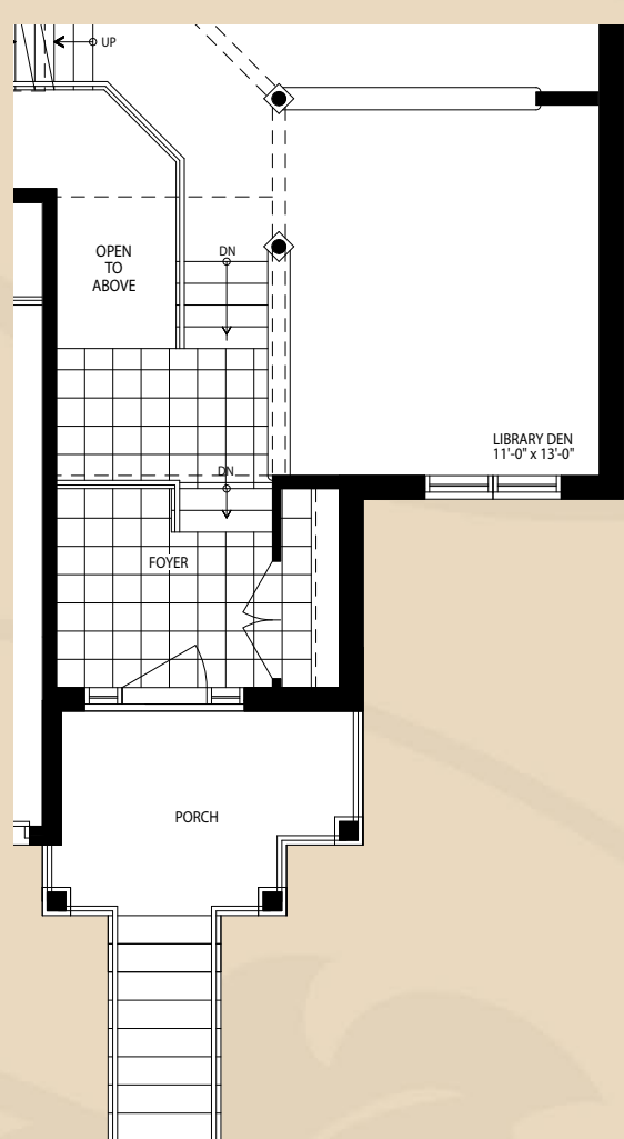
MAIN FLOOR ELEV. B1 Model for east side of Gilchrist Court Split level with library/den at kitchen level
