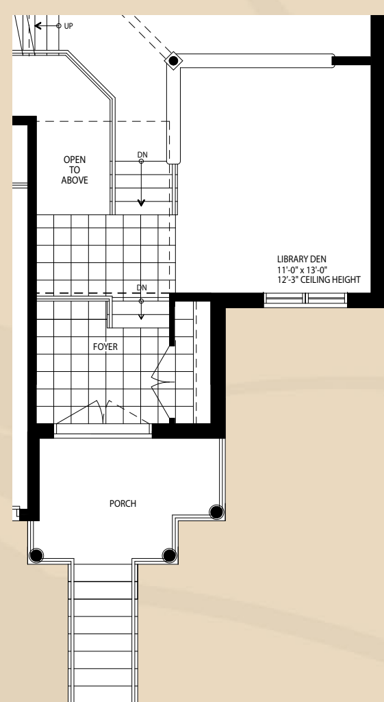
MAIN FLOOR ELEV. A2 Model for east side of Gilchrist Court Split level with library/den at laundry room level
